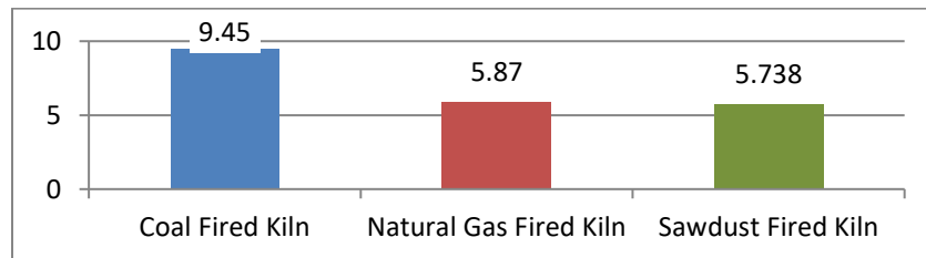
Figure 3: Comparison between Emission of PM 10 (Ton/yr)
