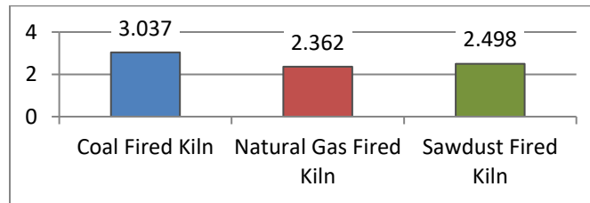
Figure 7: Comparison between Emission of NO x (Ton/yr)
