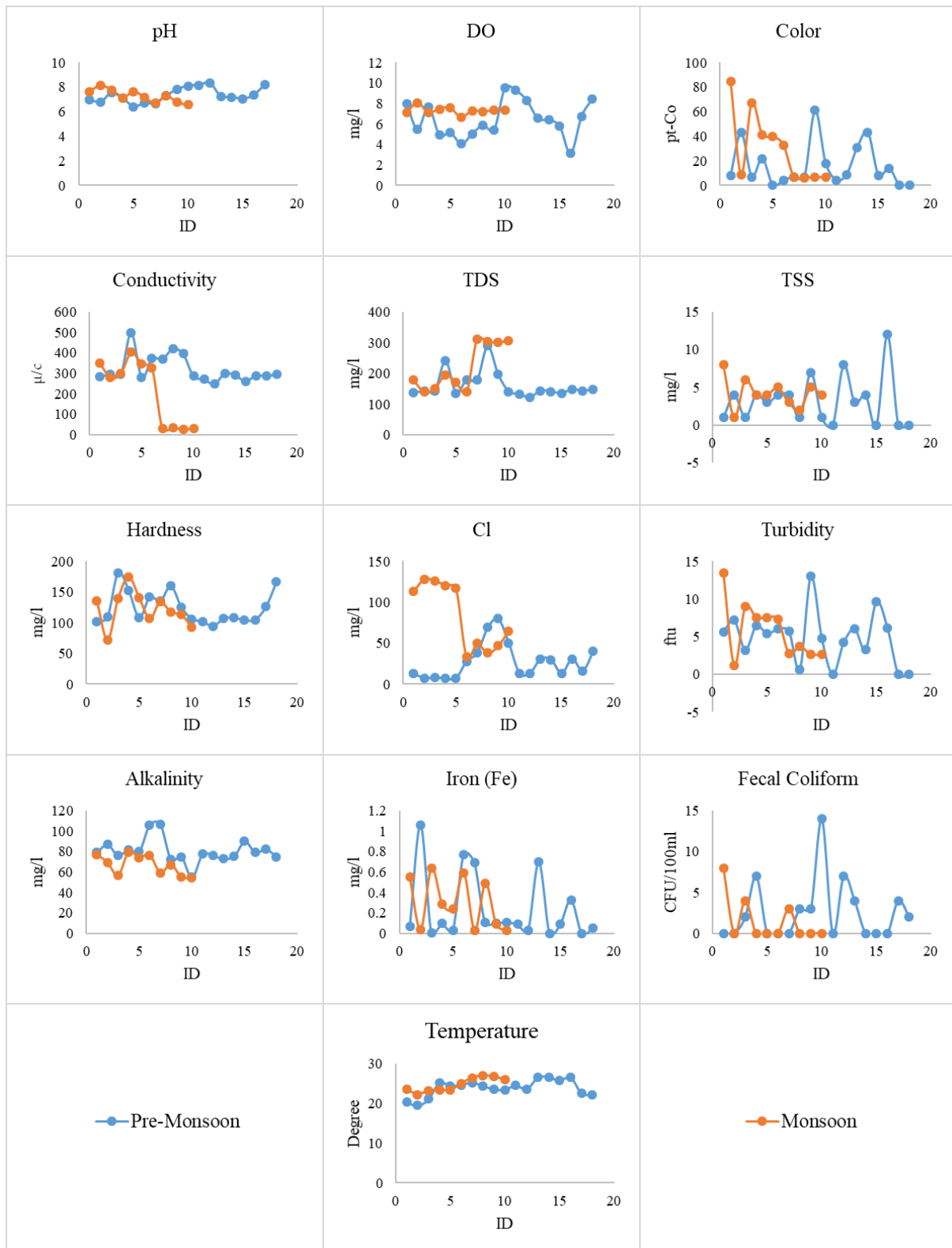
Figure 8: Variation of water quality parameters in monsoon and pre-monsoon seasons.
