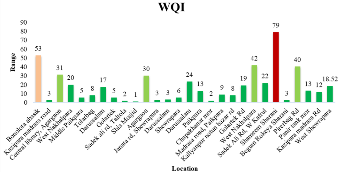
Figure 5: Water quality index and its range (WASA water).
