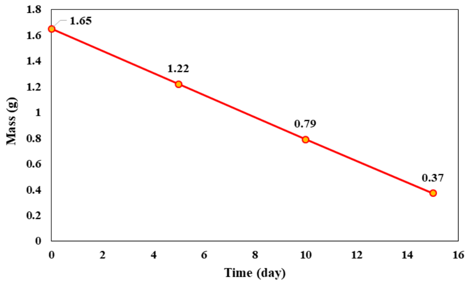
Figure 3. Biodegradability test of the film
