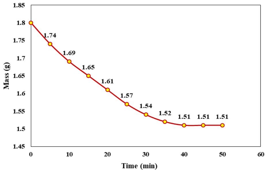
Figure 2. Depletion of mass of the composite film at 100°C for moisture content measurement
