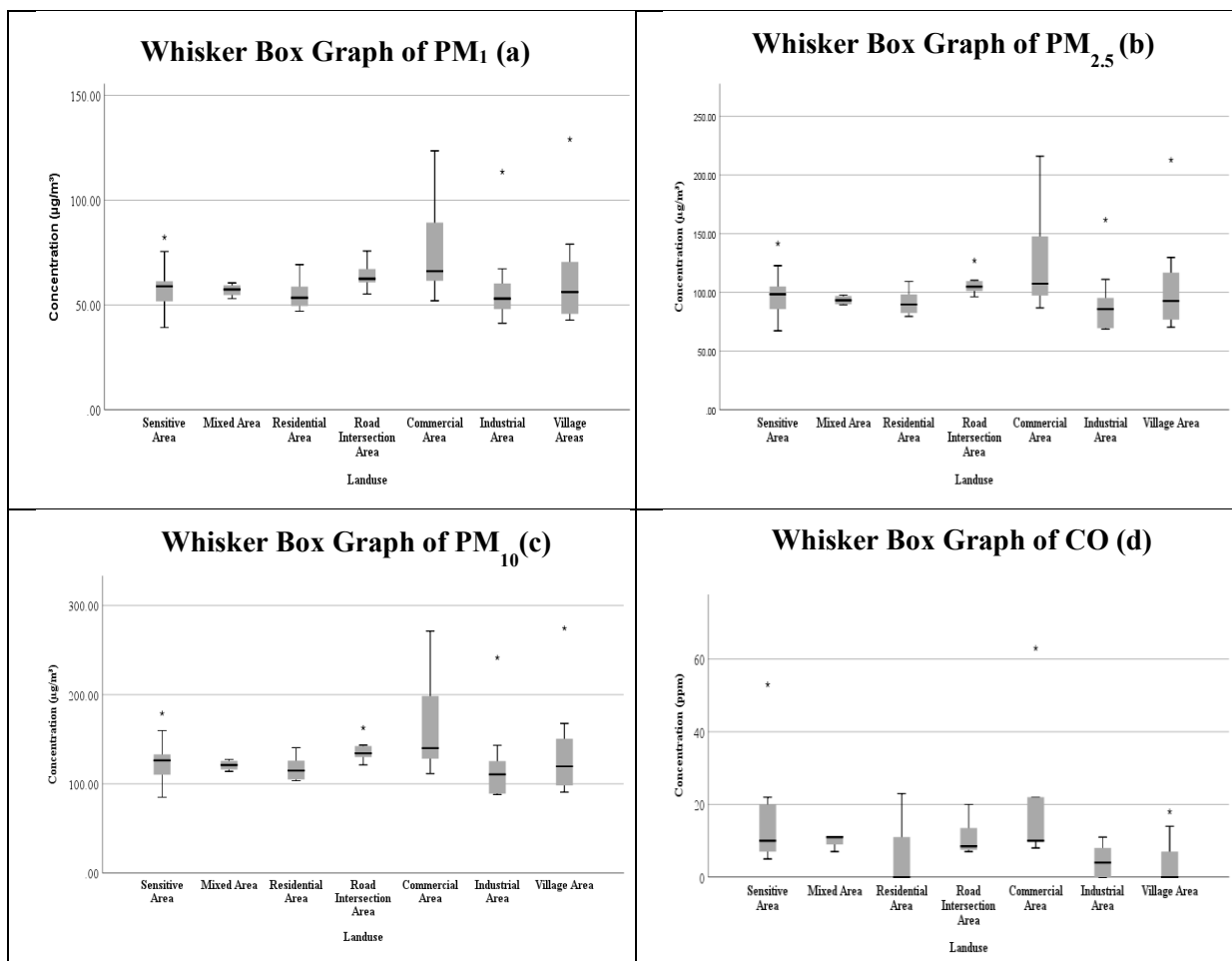
Figure 3 Whisker box plot for concentration of PM 1 , PM 2.5 , PM 10 and CO in Different Land use
