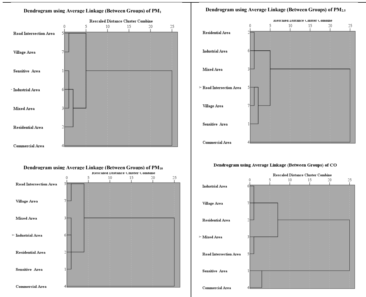
Figure 4 Land Use Based Cluster Analysis for PM 1 , PM 2.5 , PM 10 and CO
