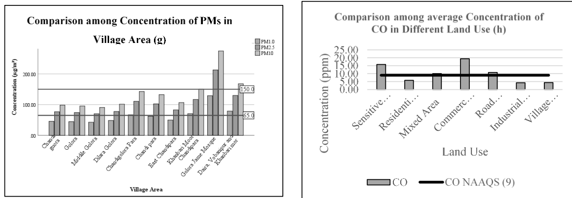
Figure 2 Comparison among Concentration of PMs and CO in Different Land Use
