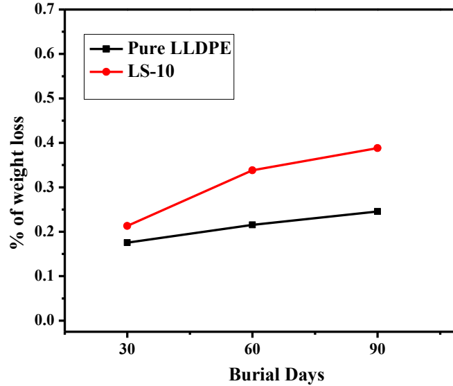
Figure 4 Soil burial test of the films
