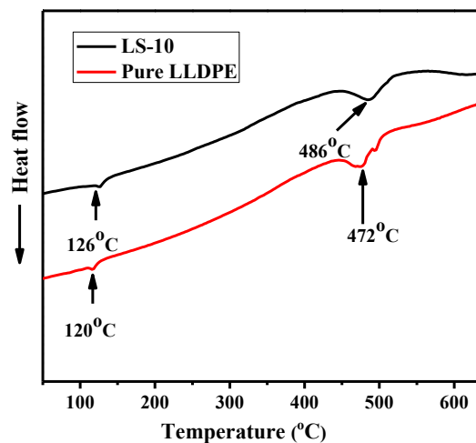
Figure 2 DSC studies of pure LLDPE film and LS-10 composite films
