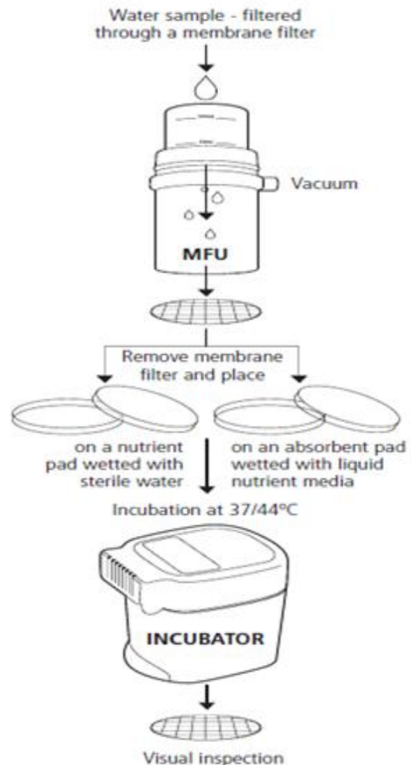
Figure 2 Preparation of Filtration unit
