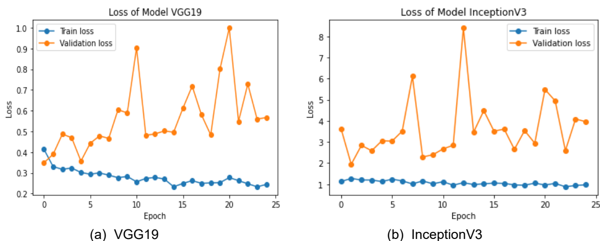
Figure 3 Loss of VGG19 and InceptionV3 models
