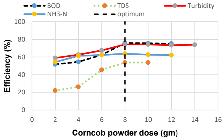
Figure 5 Effect of doses of Corncob powder on the removal of pollutant in the leachate
