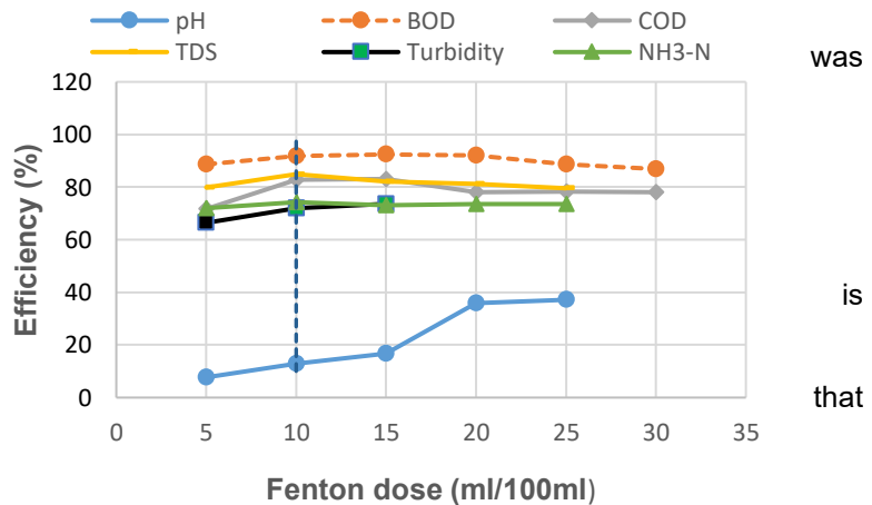
Figure 4 Effect of doses of Fenton on the removal of pollutant in the leachate.
