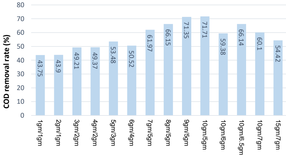
Applied doses of Hydrogen per-oxide and Ferrous sulphate (gm/gm) Figure 3 Selection of H 2 O 2 and FeSO 4 doses for Fenton reagent
