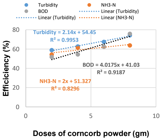
Figure 7(a) Regression analyses for treating Turbidity, NH 3 -N and BOD from leachate using Corncorb powder at various doses until the optimum
