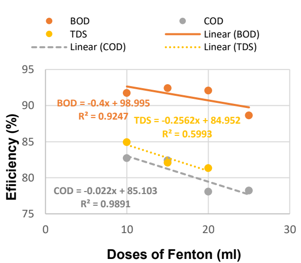
Figure 6(b) Regression analyses for treating BOD, COD and TDS from leachate using Fenton at various doses after the optimum.
