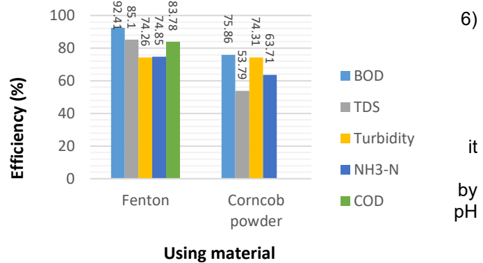
Figure 9 Optimum results of leachate treatment by Fenton and Corncob powder at optimum conditions
