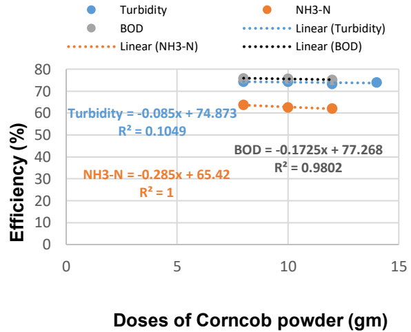
Figure 7(b) Regression analyses for treating Turbidity, NH 3 -N and BOD from leachate using Corncorb powder at various doses after the optimum
